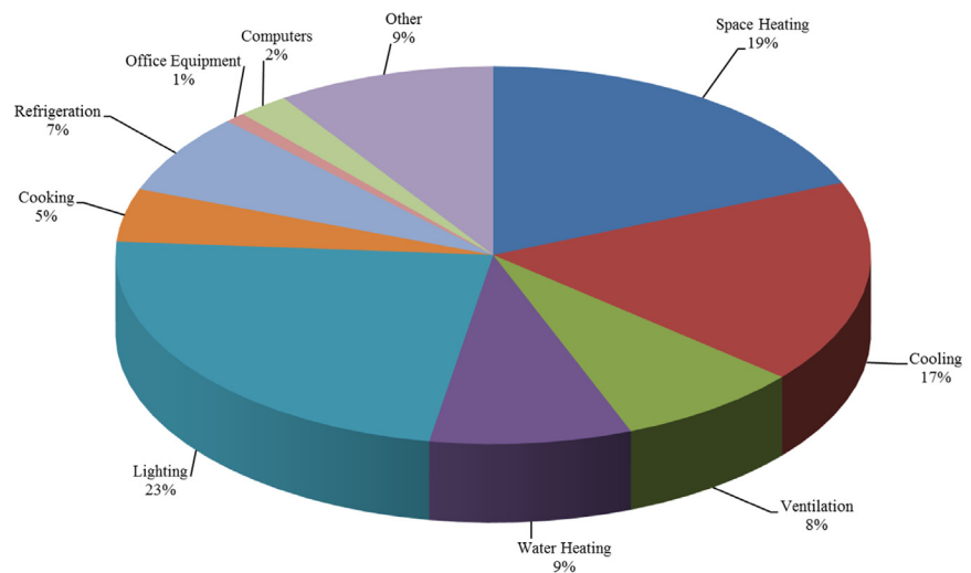
Figure 3-3b. Commercial building energy end-use estimates for cooling-dominated climates (EIA 2003).
